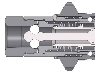
HT-Series ISO16028 Flushface Interchange Coupler with Flange Sleeve
