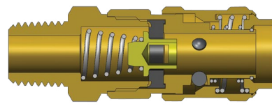
A-Series Compact Coupler (Male Threads)
