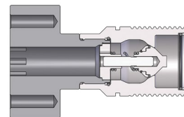
WS-Series Heavy-Duty Wingstyle Code 62 Flange Pad Plug
