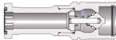
WS-Series Heavy-Duty Wingstyle Code 62 Flange Head Plug
