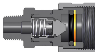
T-Series 10K Threaded Poppet Coupler (Male Threads)
