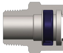
Dix-Lock N-Series Coupler (Male Threads)
