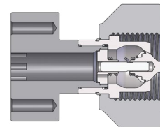
WS-Series Heavy-Duty Wingstyle Code 62 Flange Pad Coupler
