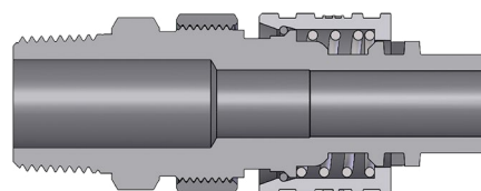
Dix-Lock N-Series Interchange Plug with Steel Locking Sleeve (Male Threads)
