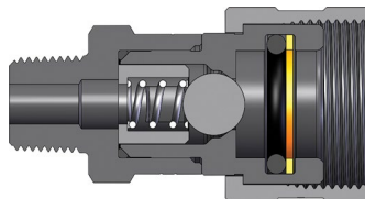
T-Series 10K Threaded Ball Coupler (Male Threads)
