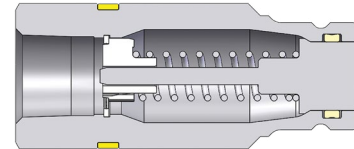
XK-Series 10K Flushface Plug (Female Threads)
