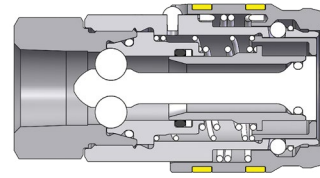
XK-Series 10K Flushface Coupler (Female Threads)
