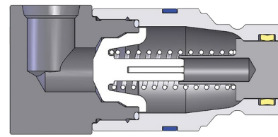
HT-Series Flushface 90° Female Threaded Plug
