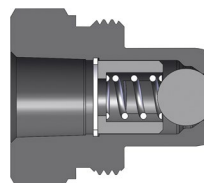
T-Series 10K Threaded Ball Plug (Female Threads)
