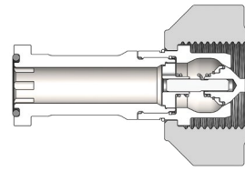
WS-Series Heavy-Duty Wingstyle Code 62 Flange Head Coupler
