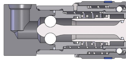
HT-Series Flushface 90° Female Threaded Coupler
