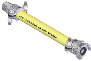
Whip Hose fitted with Heat Treated Nipple & A-Type Coupling
