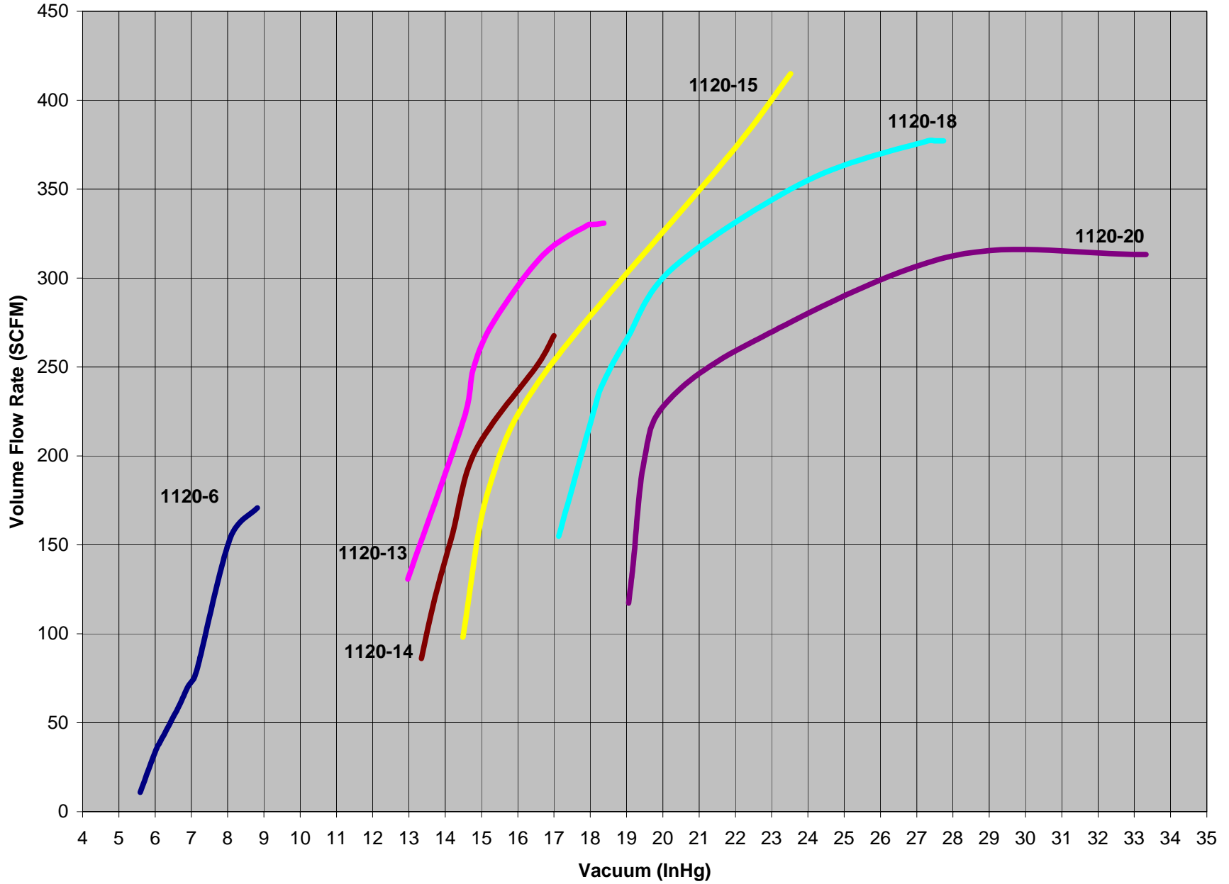
1120 Vacuum Relief Valve - Flow Rate Vs Vacuum
